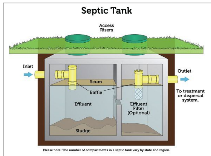
Above: A typical septic tank. Image courtesy of US EPA. Below: A conventional on-site wastewater treatment system, including a septic tank and gravel drainfield. Image courtesy of US EPA.
